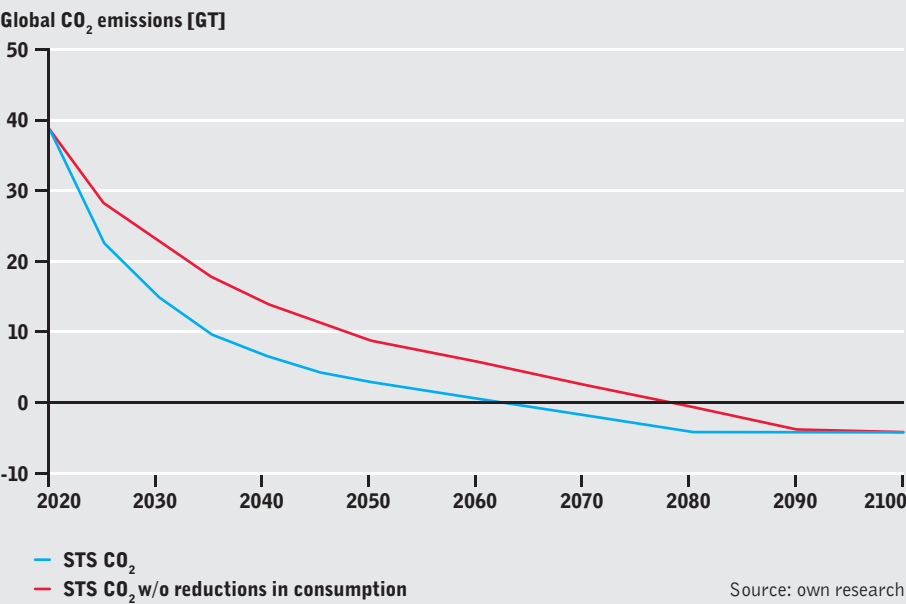
Figure 11: Comparison of global CO 2 emissions with and without reductions in consumption
